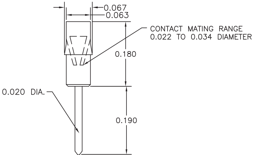
8114 SERIES RECEPTACLE CONTACT FOR: PLCC, LCC, PGA, AND OTHER LARGE PITCH SOCKETS.
