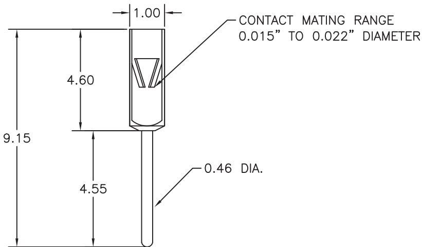
0461 SERIES RECEPTACLE CONTACT FOR: QFP, SSOP, TSOP, AND OTHER 2 AND FOUR SIDED SOCKETS.
