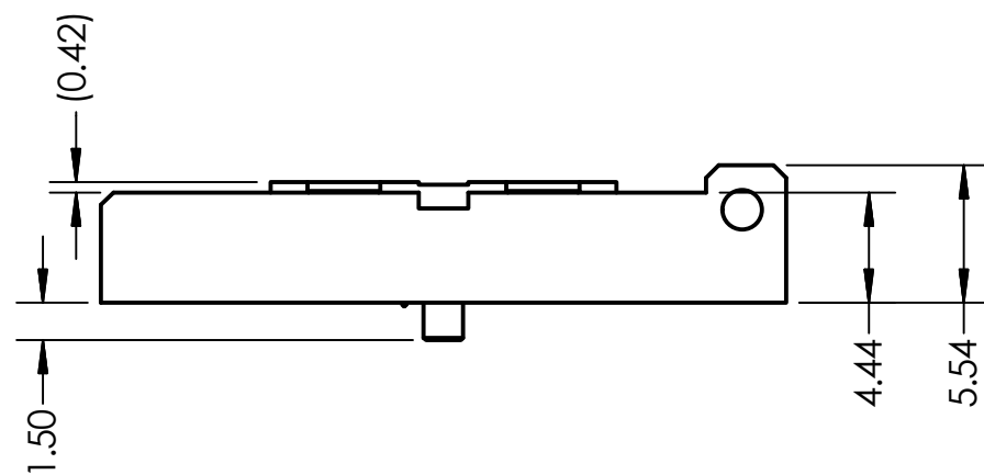
SIDE VIEW SCALE 3 : 1
