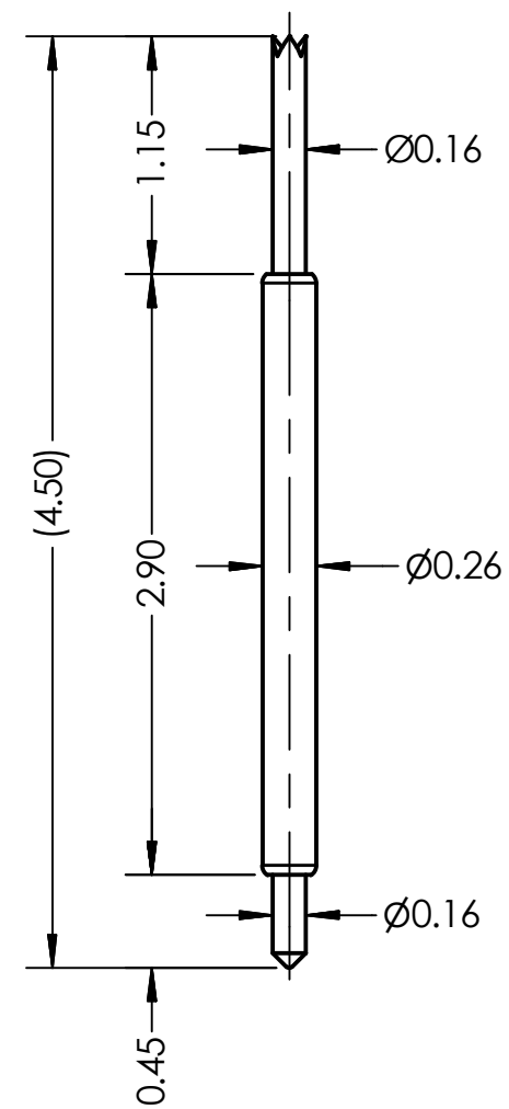
PIN CONTACT DETAIL CS1077-C
