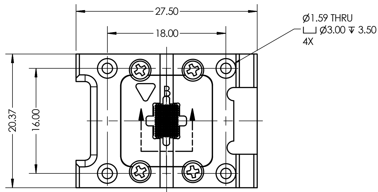
TOP VIEW SCALE 3 : 1
