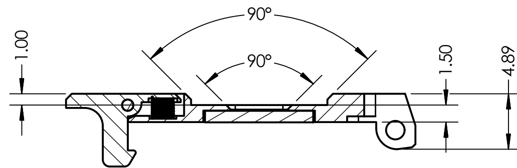
SECTION C-C SCALE 3 : 1
