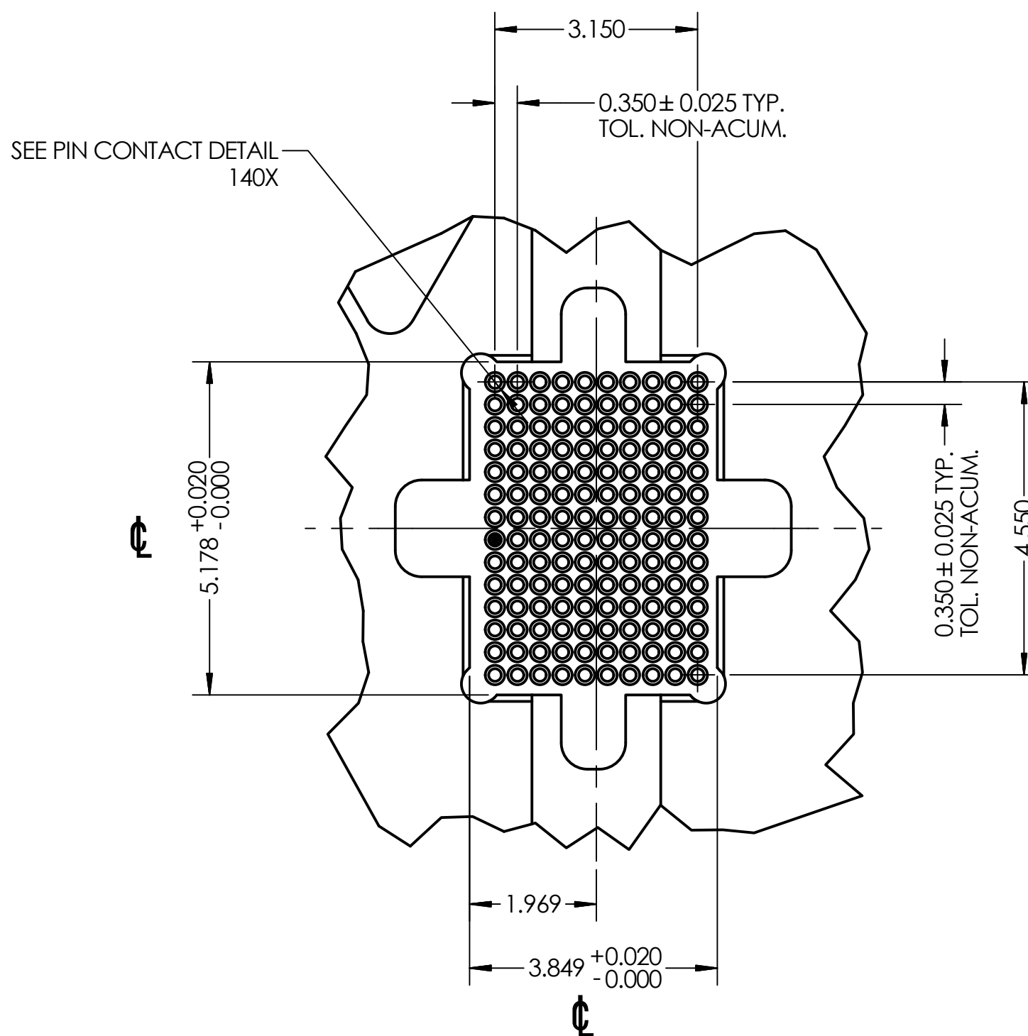
DETAIL B
