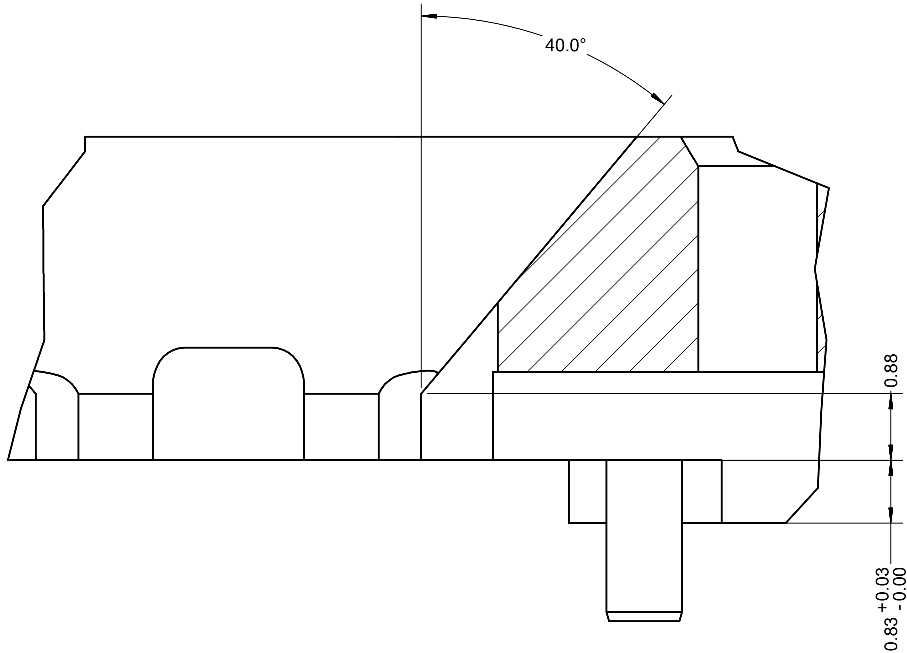
DETAIL D SCALE 20 : 1
