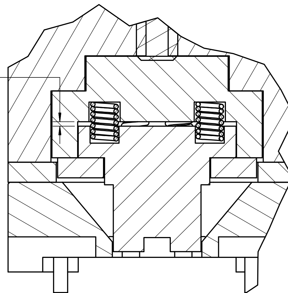
DETAIL F SCALE 8: 1
