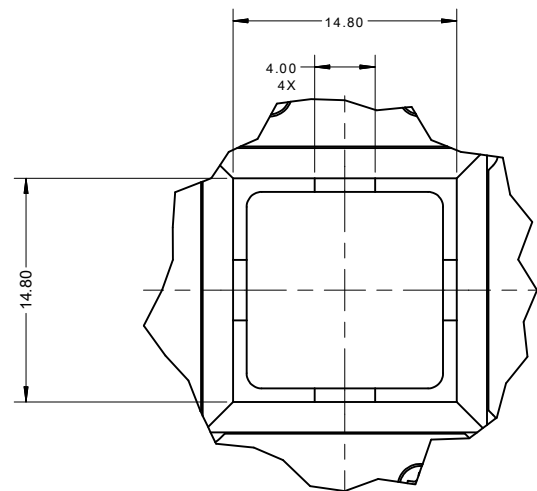
DETAIL E SCALE 4 : 1
