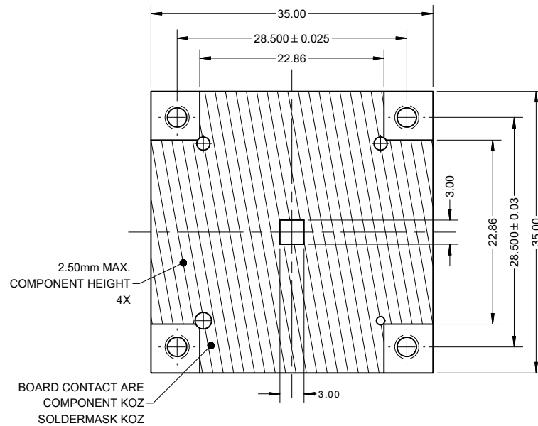
BOTTOM VIEW SCALE 3 : 1
