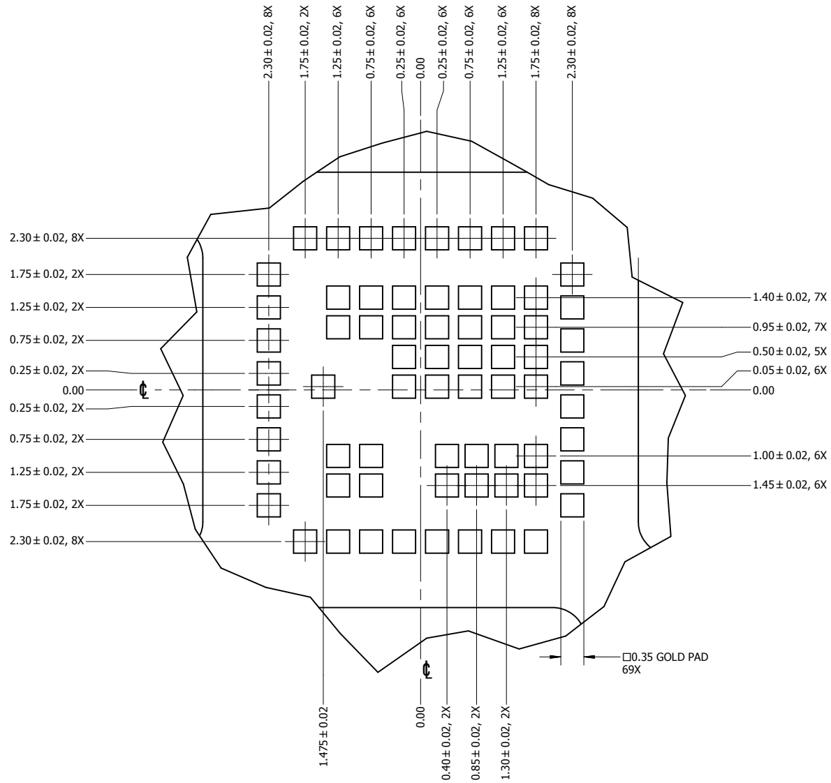
DETAIL A SCALE 25: 1
