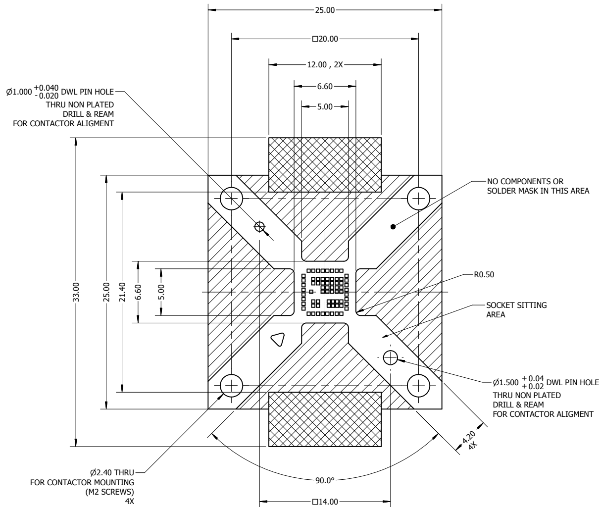
TOP VIEW SCALE 5 : 1
