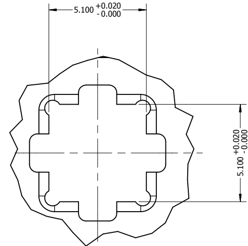
DETAIL B SCALE 10 : 1
