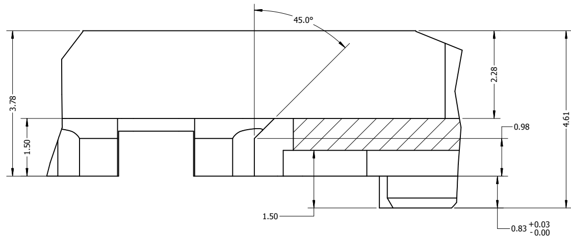
DETAIL E SCALE 20 : 1
