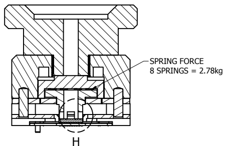
SECTION G-G SCALE 2.5 : 1
