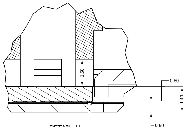
DETAIL H SCALE 17: 1
